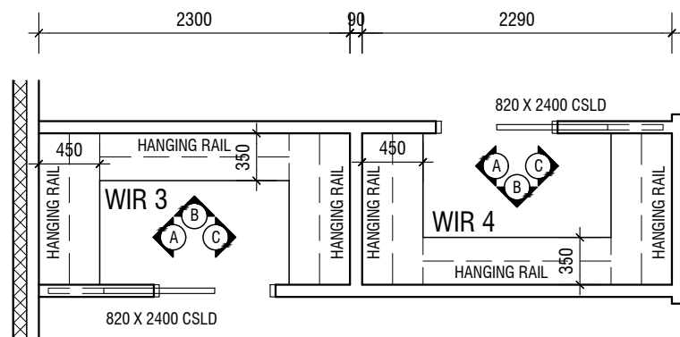
BED 3 & 4 - WALK IN ROBE PLAN
