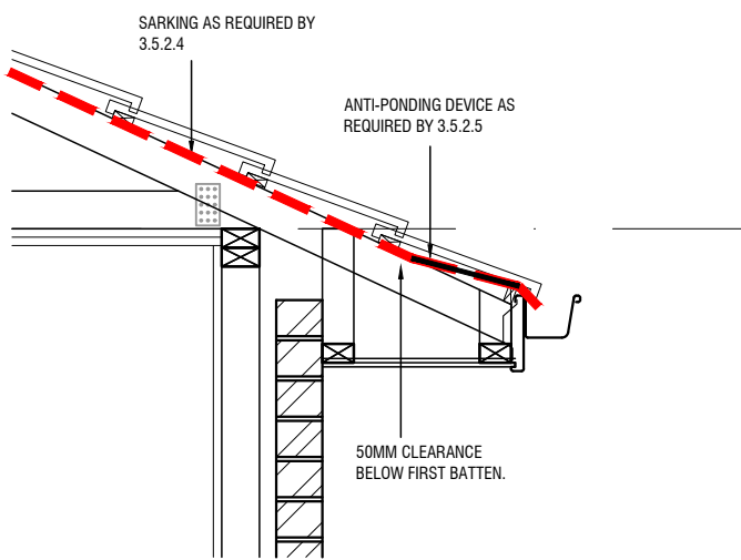
ANTI - PONDING DEVICE BOARD DETAIL - TYPICAL
