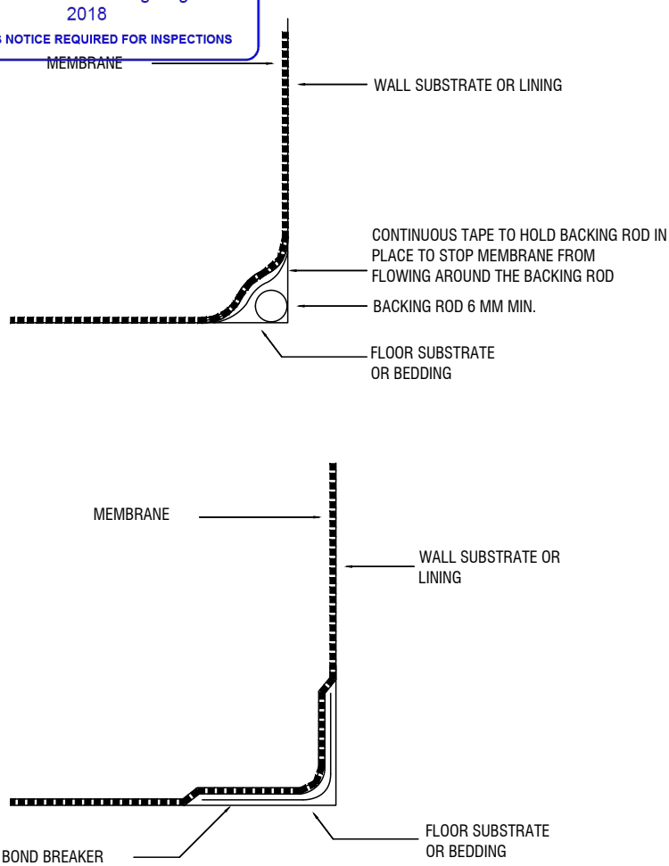
FIGURE 10.2.27: EXPLANATORY: TYPICAL BOND BREAKER DETAILS
