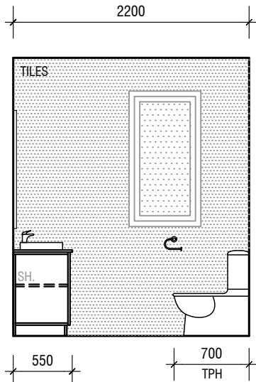
ELEVATION C
