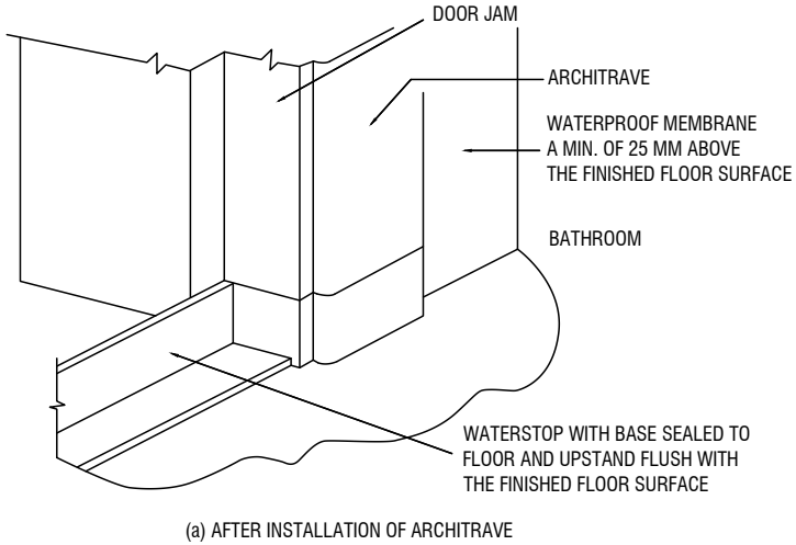
FIGURE 10.2.24: TYPICAL BATHROOM DOOR DETAILS FOR WHOLE BATHROOM WATERPROOFING
