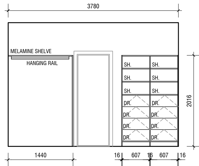
ELEVATION D
