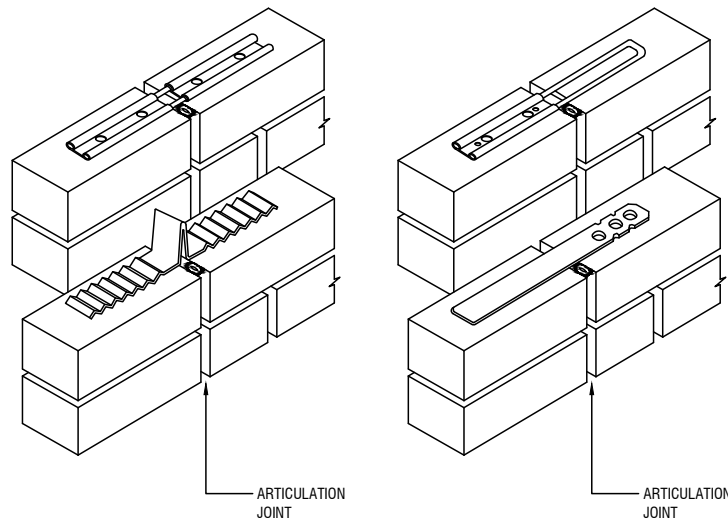
MASONRY EXPANSION (SLIDING/EXTENDABLE) TIES
