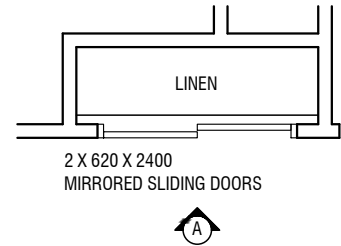
LINEN PLAN ELEVATION A
