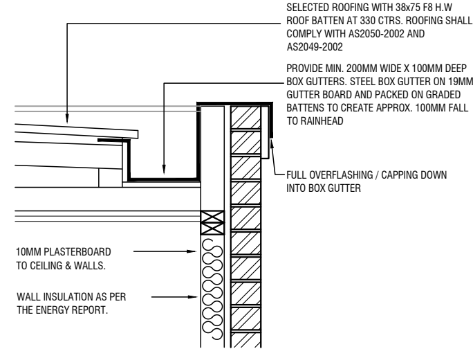
BOX GUTTER DETAIL - TYPICAL
