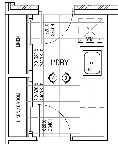
LAUNDRY PLAN
