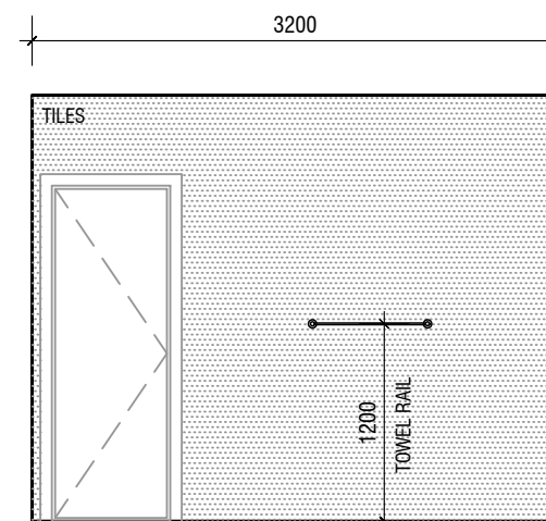
ELEVATION D
