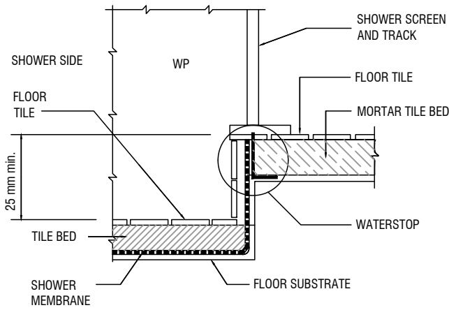
FIGURE 10.2.15A: TYPICAL ENCLOSED STEPPED DOWN SHOWER CONSTRUCTION (MEMBRANE BELOW TILE BED)
