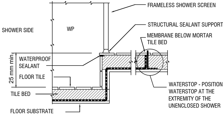
FIGURE 10.2.15C: TYPICAL UNENCLOSED STEPPED DOWN SHOWER CONSTRUCTION (MEMBRANE BELOW TILE BED)
