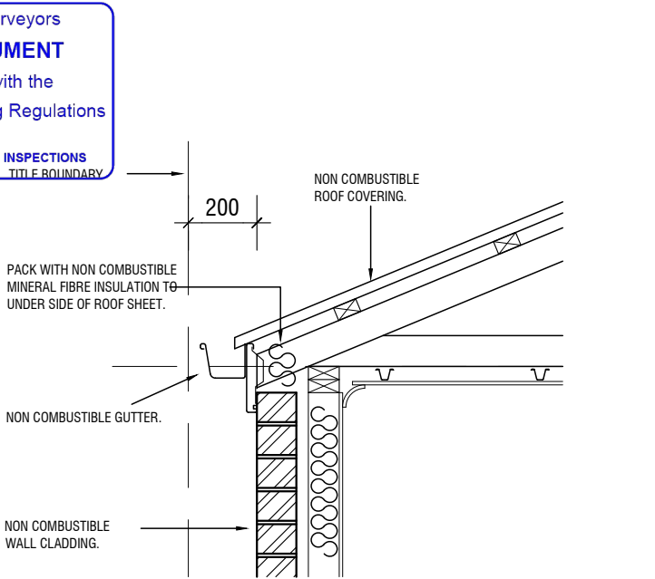
NO EAVE OVERHANG DETAIL - TYPICAL
