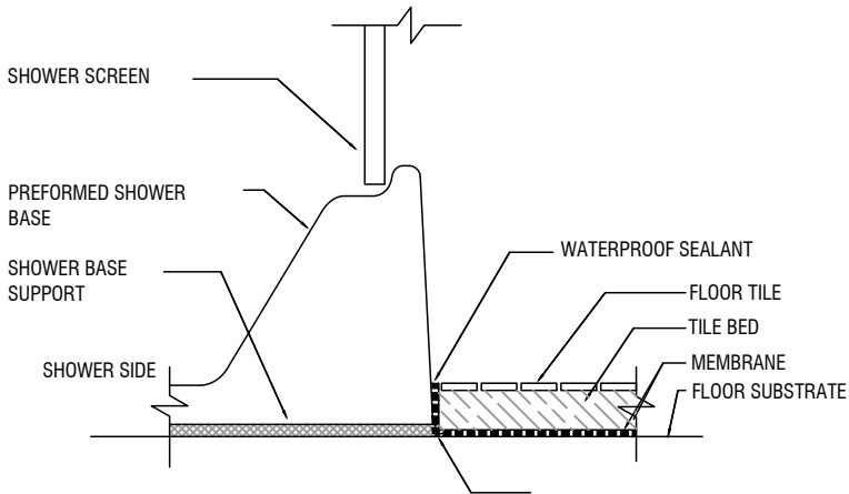
FIGURE 10.2.19B: TYPICAL PREFORMED SHOWER BASE/FLOOR JUNCTION ON TIMBER FLOORS, INCLUDING PARTICLEBOARD,PLYWOOD AND OTHER TIMBER MATERIALS
