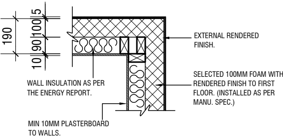
FIRST FLOOR WALL DETAIL
