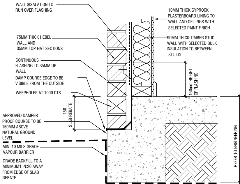
TYPICAL SLAB REBATE DETAIL
