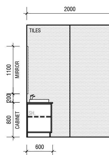
ELEVATION C
