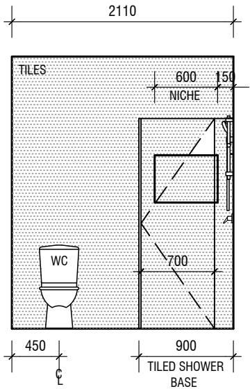
ELEVATION D
