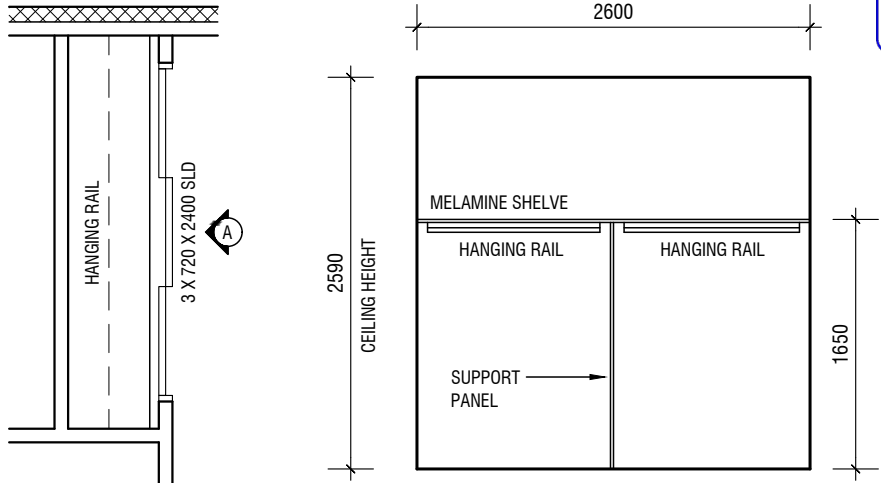
BED 5 ROBE PLAN ELEVATION A
