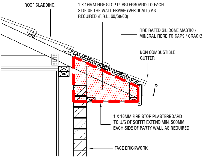
EAVE / SOFFIT SEPERATION DETAIL - TYPICAL 60/60/60
