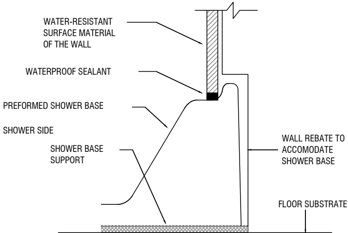
FIGURE 10.2.19A: TYPICAL PREFORMED SHOWER BASE WALL/FLOOR JUNCTION
