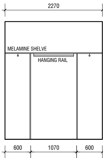
ELEVATION C
