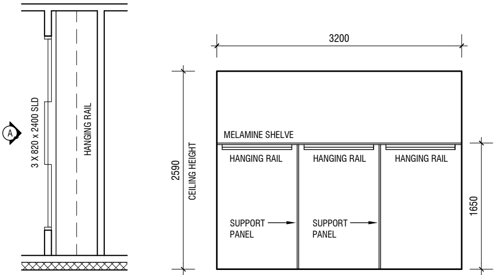
BED 2 ROBE PLAN ELEVATION A
