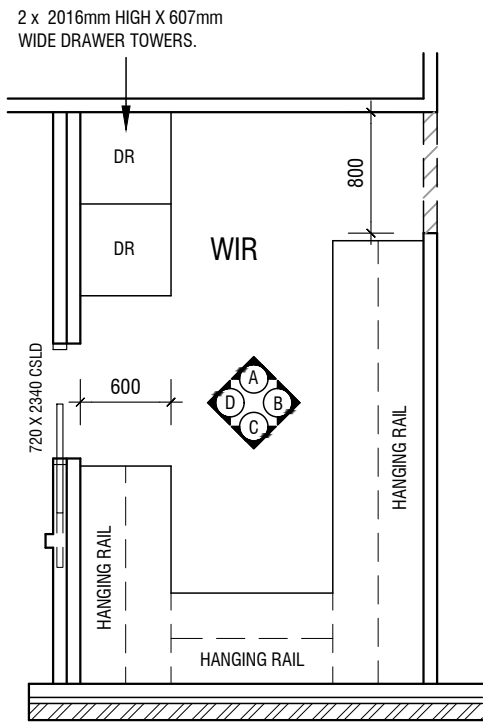
BED 1 - WALK IN ROBE PLAN
