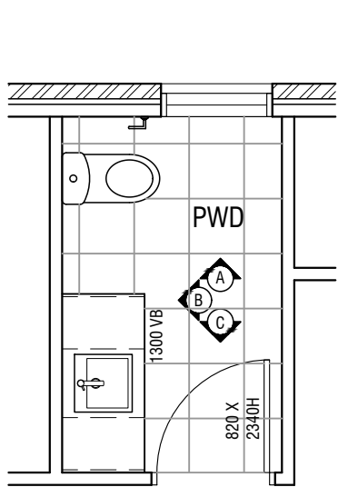
POWDER ROOM PLAN
