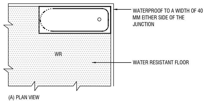
FIGURE 10.2.4A: AREAS ADJACENT TO BATHS AND SPAS WITHOUT SHOWERS FOR CONCRETE, COMPRESSED FIBRE-CE-MENTAND FIBRE-CEMENT SHEET FLOORING.
