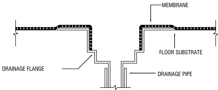
FIGURE 10.2.29: TYPICAL MEMBRANE TERMINATION AT DRAINAGE OUTLET
