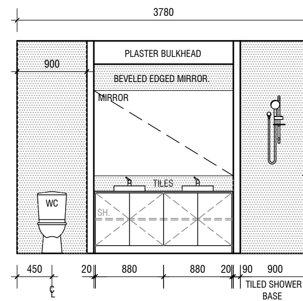
ELEVATION D
